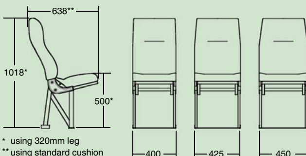
Dimensions (for guidance only)
